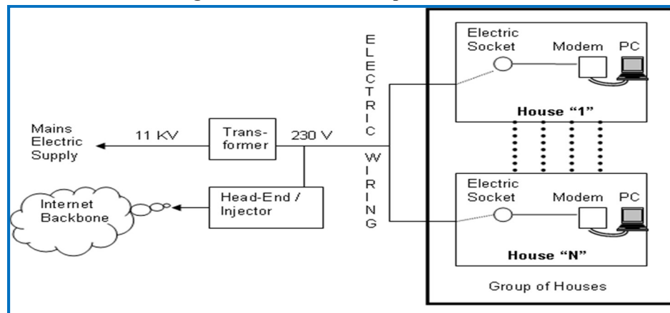
Figure 8: Broadband over power line
