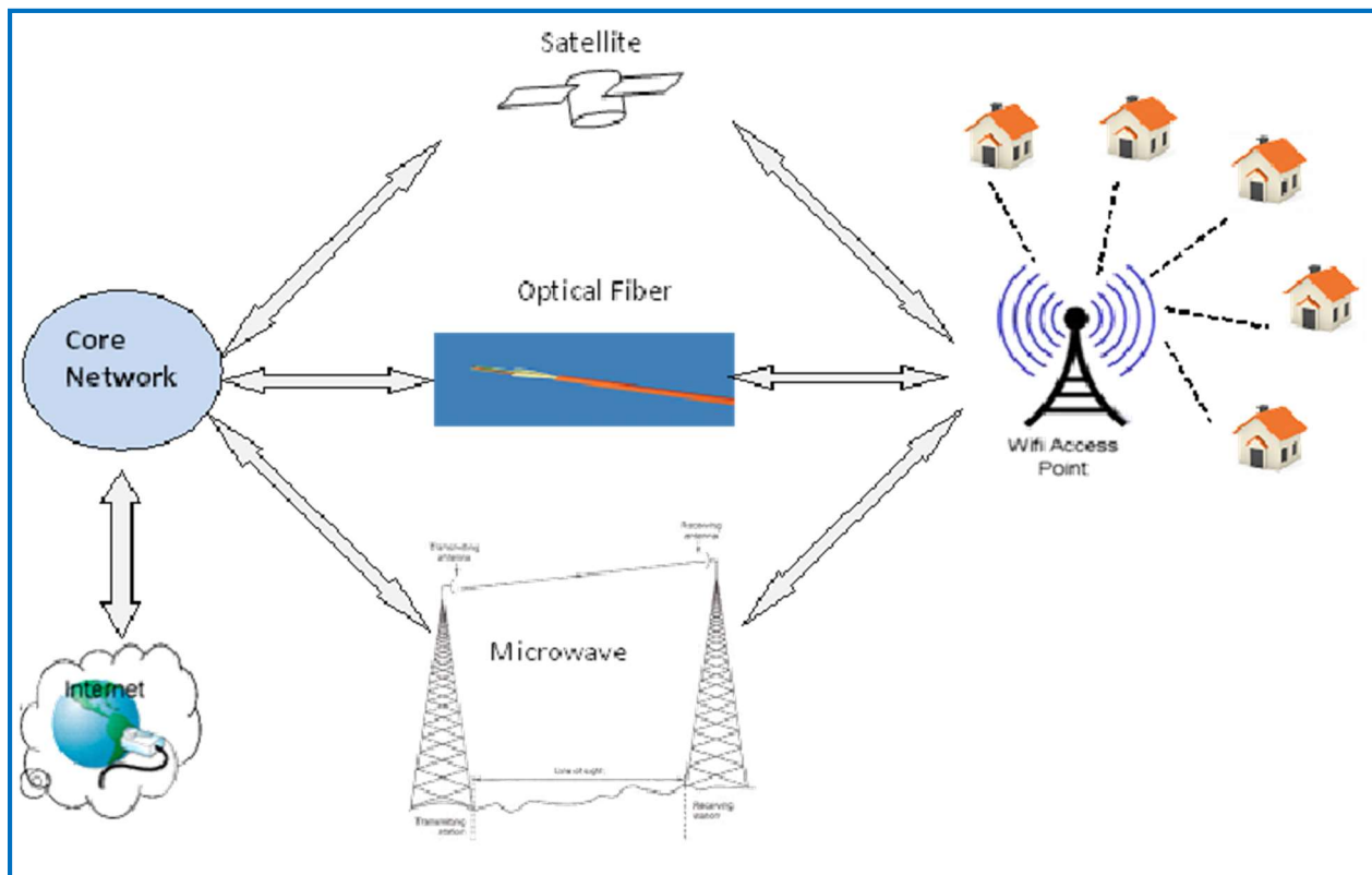
Figure 13: Technology Options for Backhaul Network
