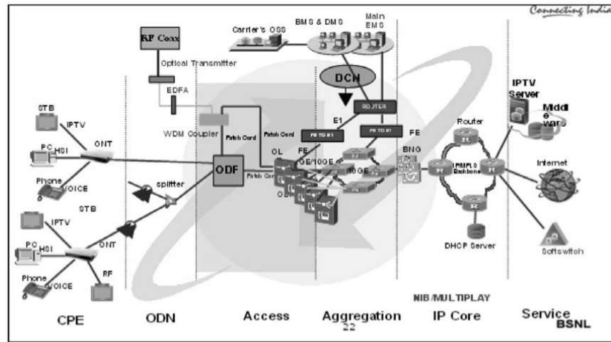
Figure 3. BSNL FTTH Architecture.
