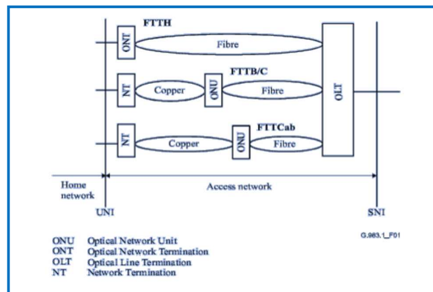
Figure 7: Network Architecture of Access Optical Network (Source: ITU-T G.983.1)
