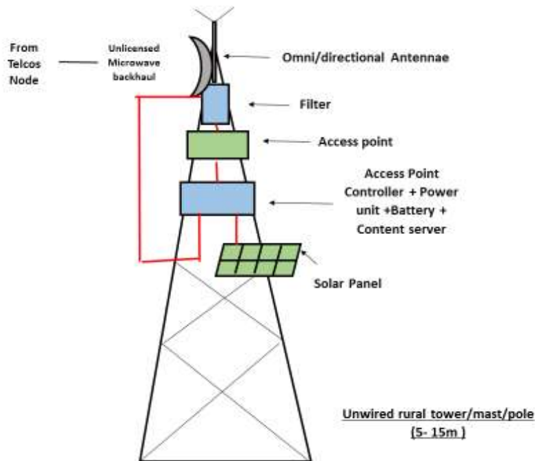
Everything on Tower(EOT) – A Schematic
